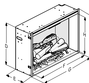
Firebox Dimensions
